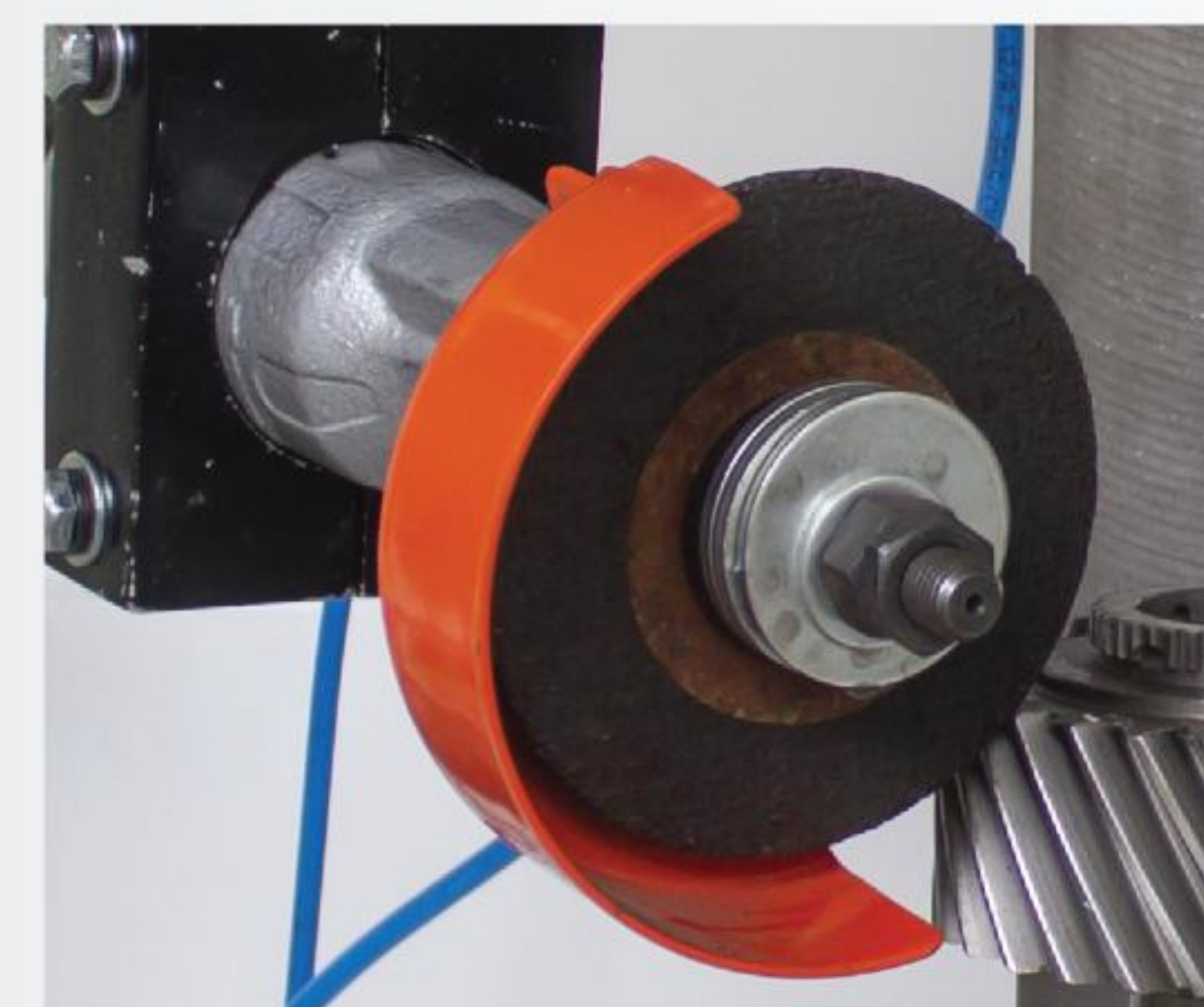
PNEUMATIC GRINDER
