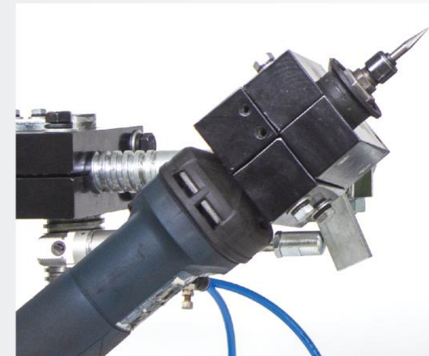
ELECTRIC GRINDER
